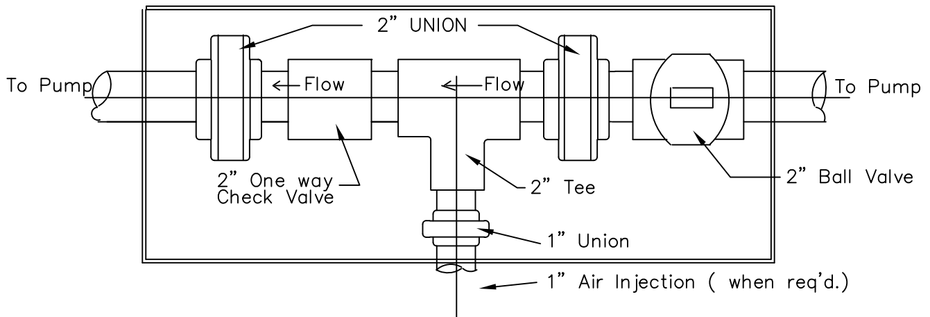
SIMPLEX STATION CONFIGURATION
