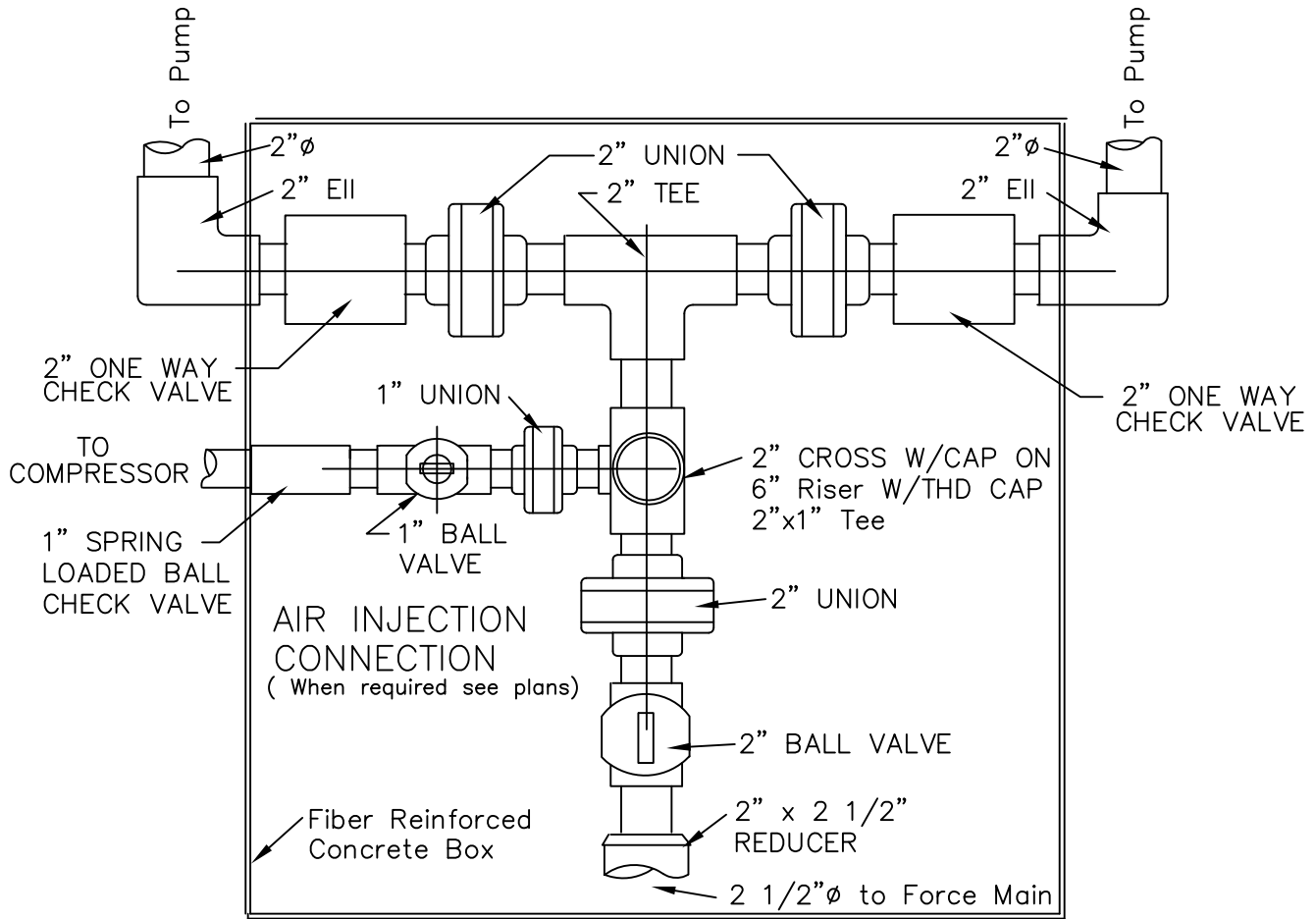
DUPLEX STATION CONFIGURATION
